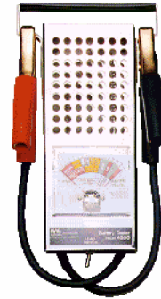
H/D Copper Plated Clamps 100 Amp Capacity Load Safety Switch For 6 & 12 Volt Batteries Tests: Voltage Supply, Cranking Volts, Charging Volts and Good/Bad Battery Test
