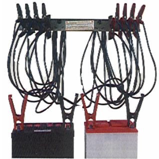
6075 - Parallel Bus Bar Charging Station
